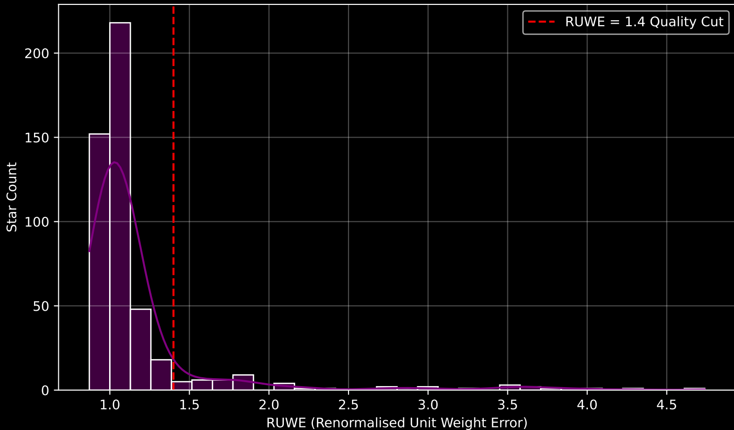
GALAH DR4 Field [9467] RUWE Distribution (n= 484)
