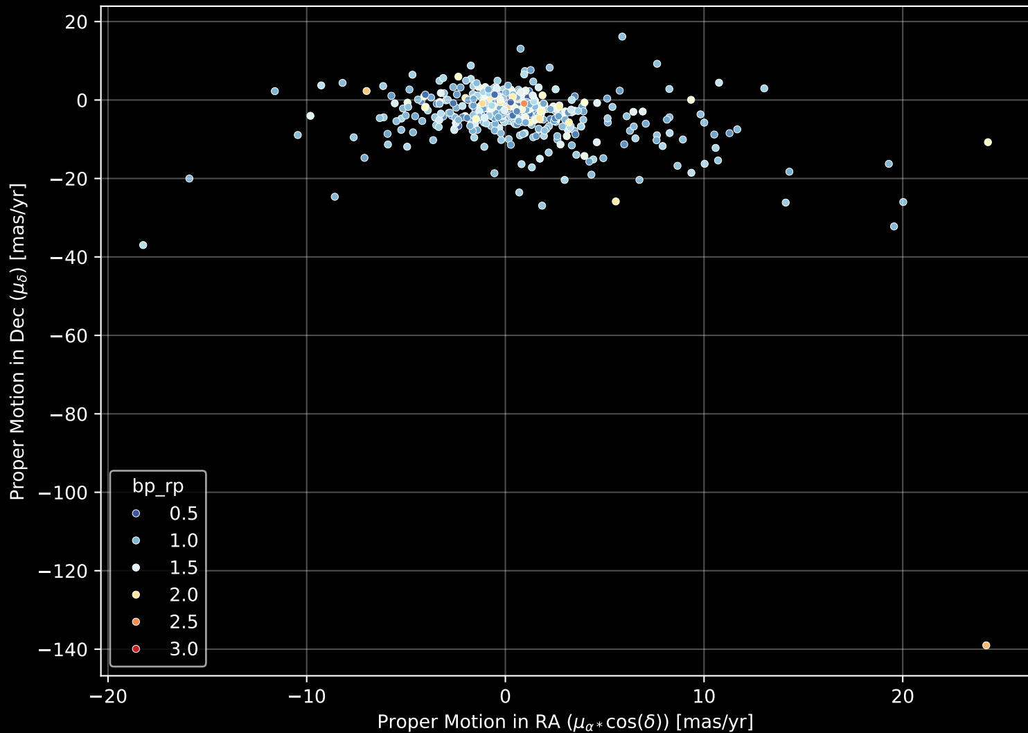
GALAH DR4 Field: [9467] Proper Motion Diagram (n= 495)
