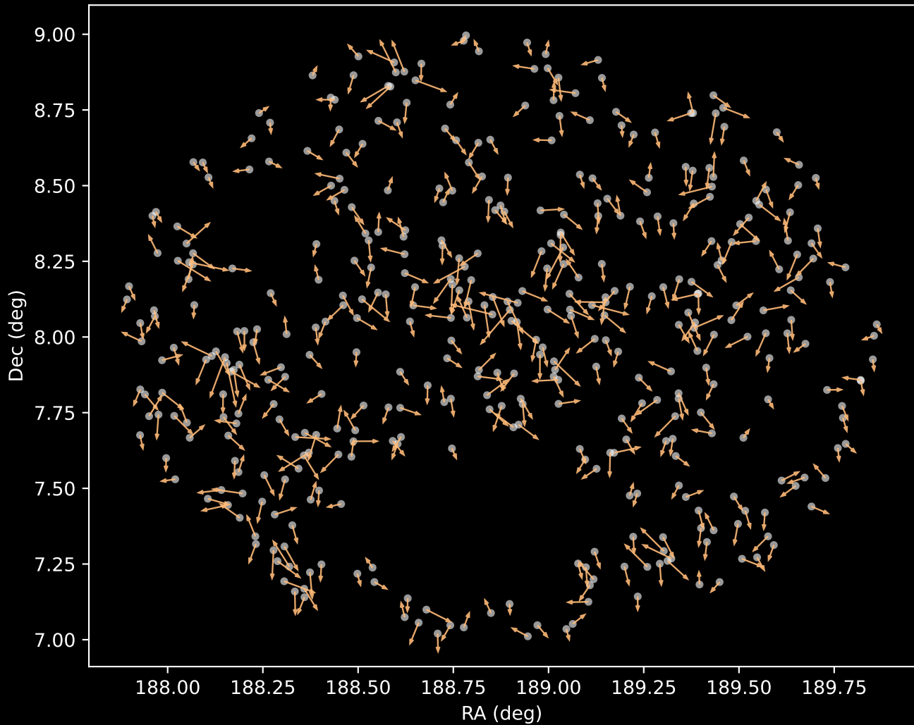
GALAH DR4 Cluster 3 Proper Motion Vectors (n=422)
