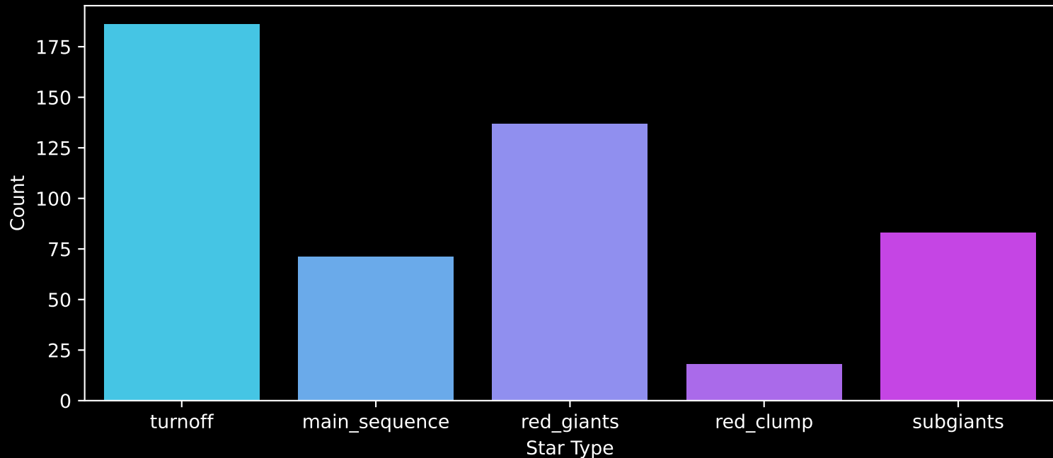
GALAH DR4 Field: [9467] Count plot of Star Type
