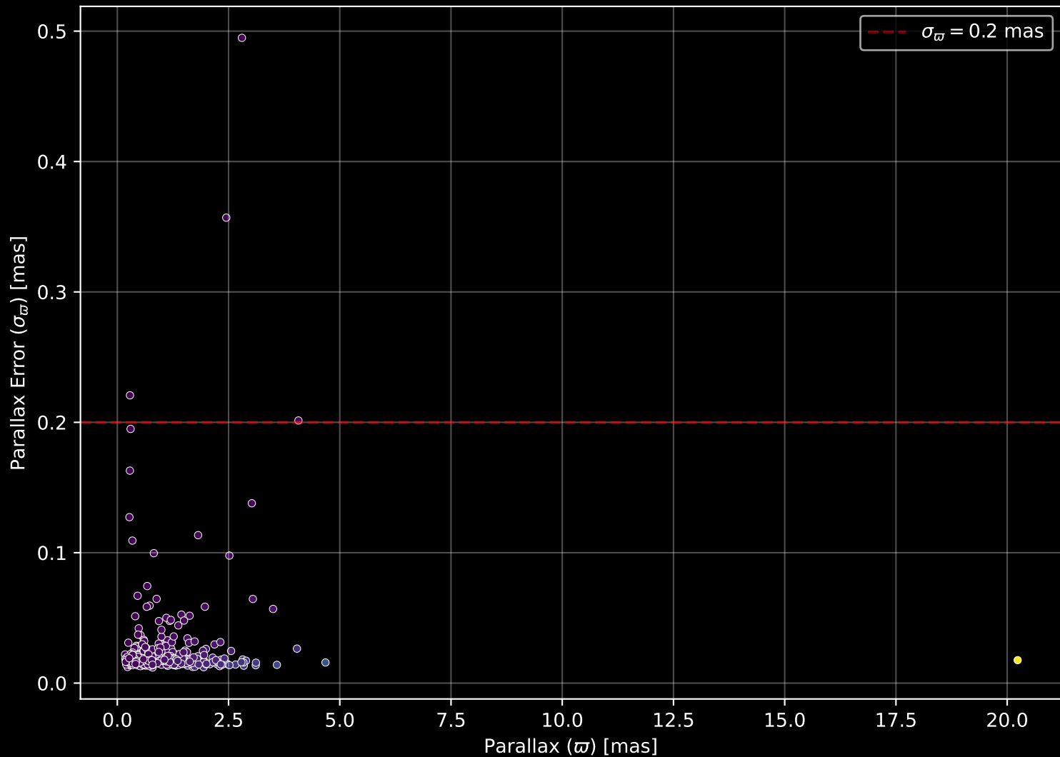
GALAH DR4 Field: [9467] Parallax Quality (n= 495)
